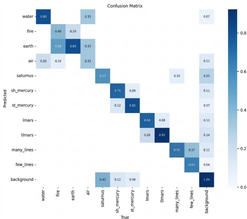
Figure 4. Confusion matrix for testing all object data
